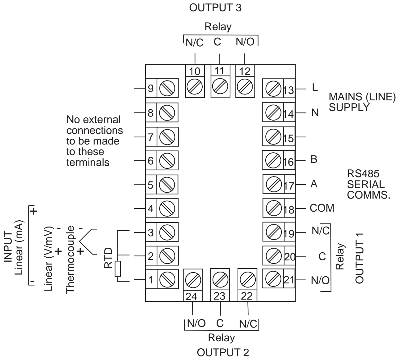
FIGURE 2-6 Wiring Label
